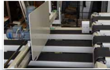
Pre-hopper with moveable gate. Gate adjustable in depth.
