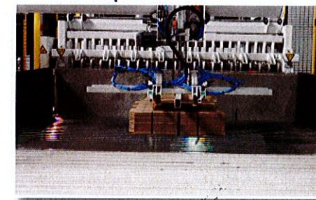
Tie sheet unit: with the ability to run also paper tiesheets
